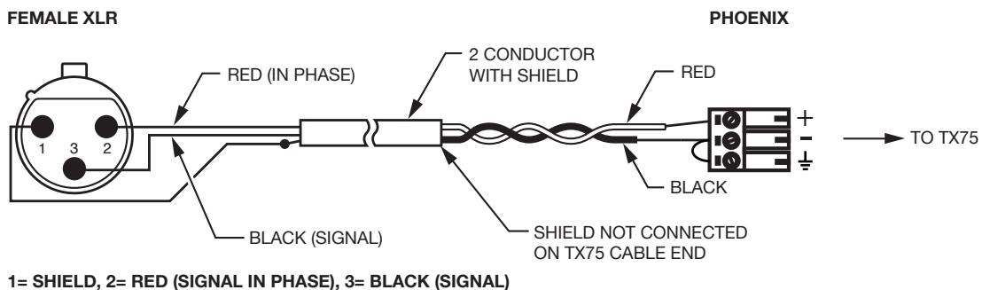
Figure 8: Unbalanced line out (XLR) to WIR TX75 C/D PRO line input (Phoenix Contact® connector) cable
