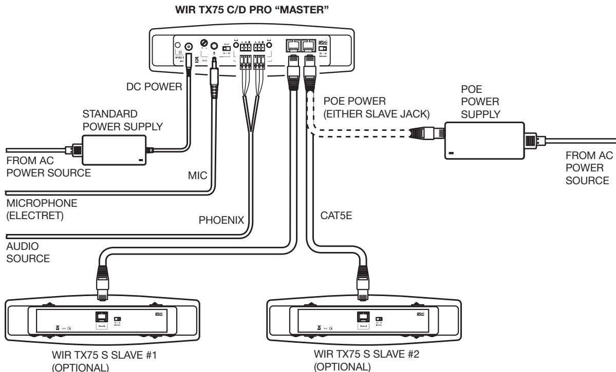
Figure 9: Connecting a WIR TX75 C/D PRO master transmitter to two WIR TX75 S slave emitters
