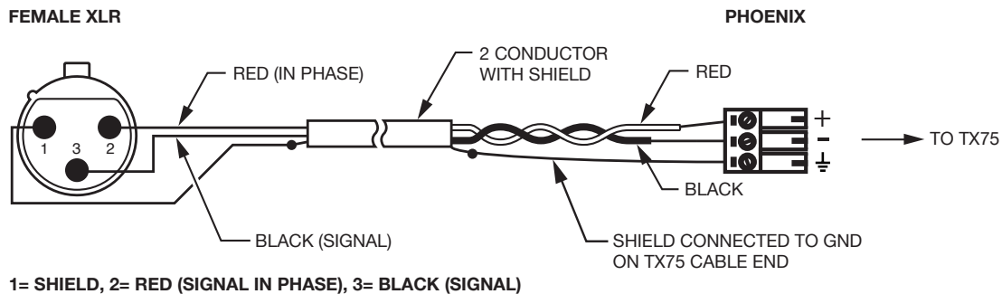
Figure 7: Balanced line out (XLR) to WIR TX75 C/D PRO line input (Phoenix Contact® connector) cable
