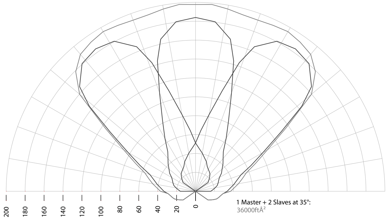
Figure 5: WIR TX75 C/D PRO master and two WIR TX75 S slaves each at an angle of 35° from the master.
