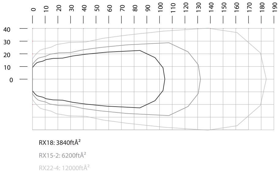
Figure 1: Receiver coverage area with WIR TX75 C/D PRO transmitter OR WIR TX75 S slave emitter in single channel mode.
